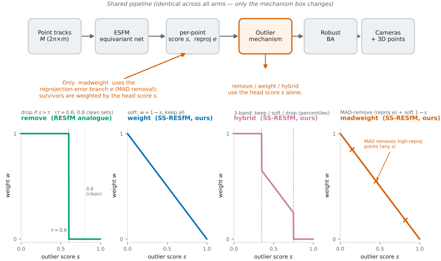
Figure 2: Method. A shared pipeline (top) in which only the outlier-mechanism block changes. The four mechanisms as weight-vs-signal transfer functions (bottom). Only madweight consumes the reprojection-error branch e , and only for its removal step; its surviving points are still weighted by the head score s ( w=1-s ). The other three mechanisms use s alone.
